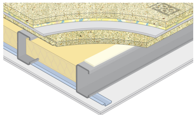
Monarfloor® Deck 18 on a timber sub-floor supported by steel joists.
