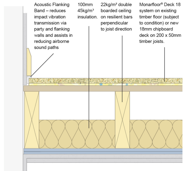
Monarfloor® Deck 18 platform floor / floating floor system on a timber sub-floor with a resilient bar system
