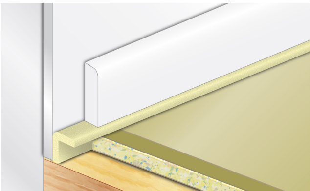
Monarfloor® Deck 18 platform floor / floating floor system on a timber sub-floor with a resilient bar system
