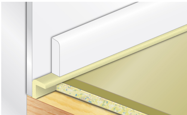
Monarfloor® Deck 22 platform floor / floating floor system on a timber sub-floor with a resilient bar system
