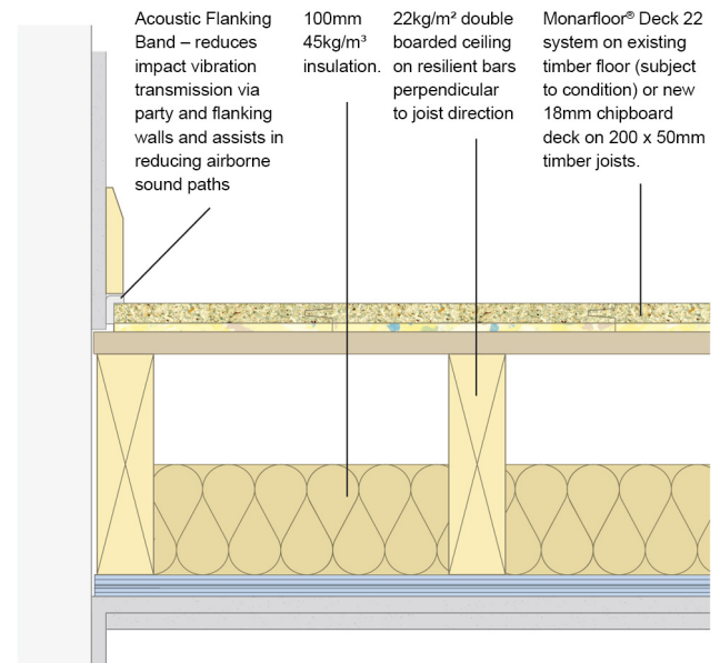
Monarfloor® Deck 22 platform floor / floating floor system on a timber sub-floor with a resilient bar system
