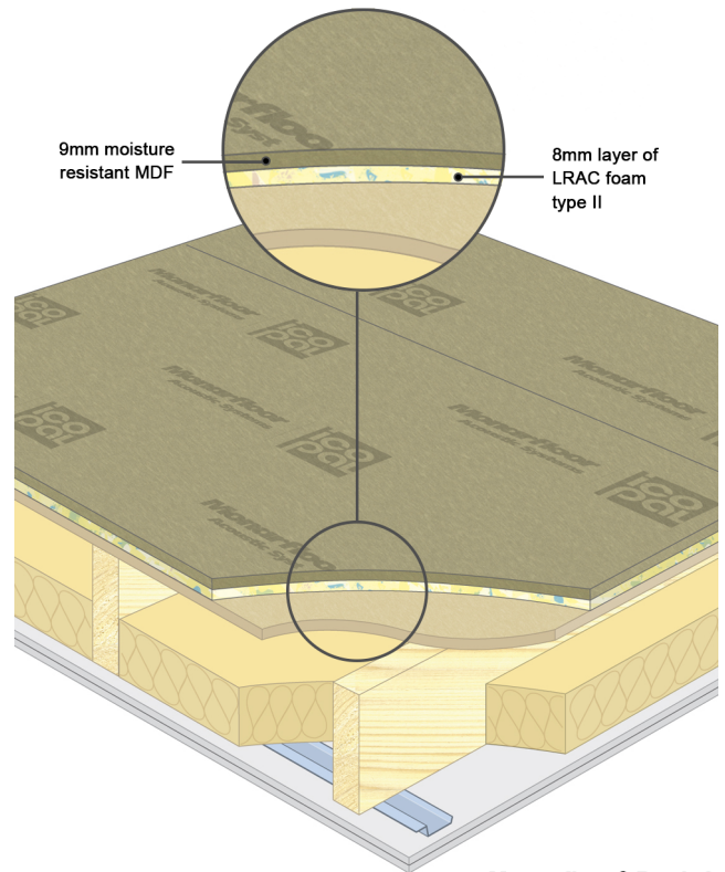
Monarfloor® Deck 9 on a timber sub-floor
