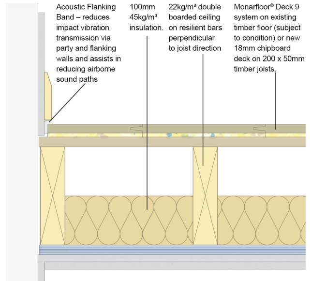
Monarfloor® Deck 9 platform floor / floating floor (FFT5) system on a timber sub-floor with a resilient bar system
