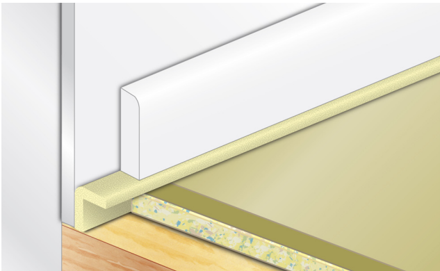
Monarfloor® Deck 9 platform floor / floating floor (FFT5) system on a timber sub-floor with a resilient bar system
